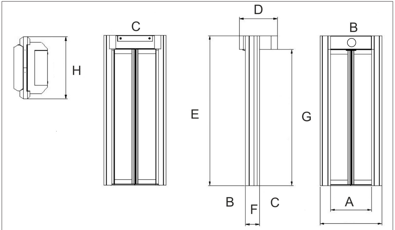
FlipFlow WIDE dimensions (millimetre / inch)
